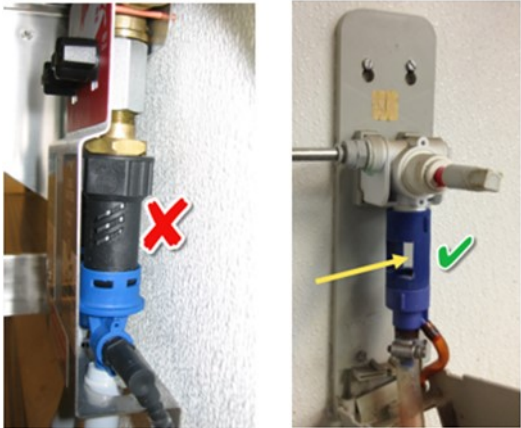
Figure 2 – ASSE 1055 Air Gapped Equipped
