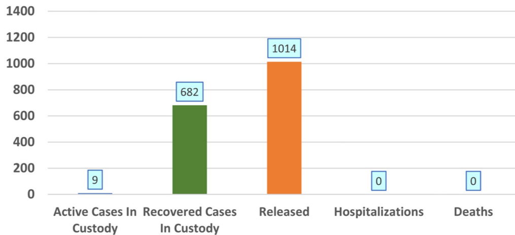
Distribution of Positive Cases as of 11/24/2020
