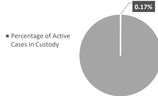
Percentage of Jail Population with COVID-19 as of 11/24/2020
