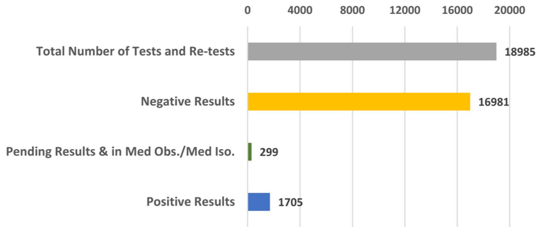
COVID-19 Testing and Results as of 11/24/2020
